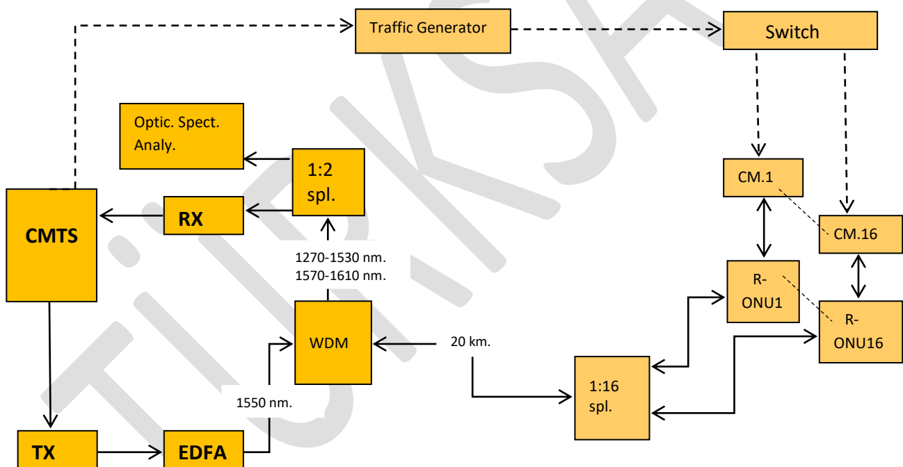
Figure-1 :OBI-FREE RFOG NODE TEST SET-UP
