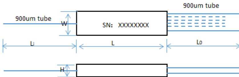
Figure 1 Definition of ports on a mini-module PLC splitter without connector
